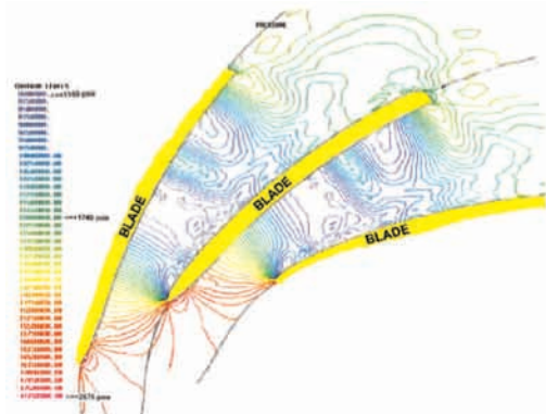
Figure 11. Impeller Static Pressure Distribution During Overload Operation.
