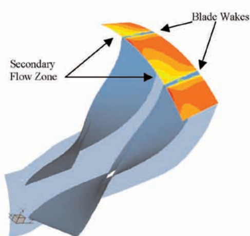
Figure 10. Impeller Blade Wakes.
