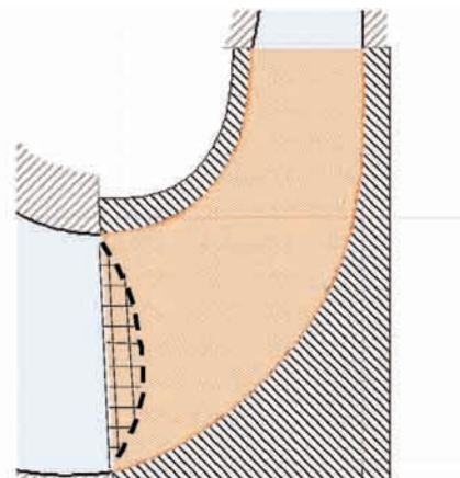
Figure 4. Schematic of Blade Leading Edge Fracture
