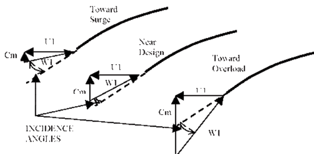
Figure 5. Impeller Incidence.
