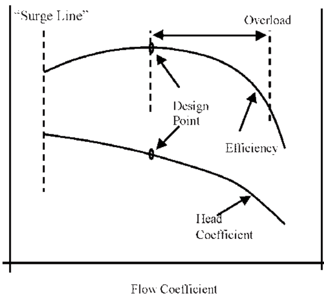
Figure 1. Definition of Overload.
