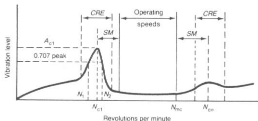
Critical Speed Separation Margins
