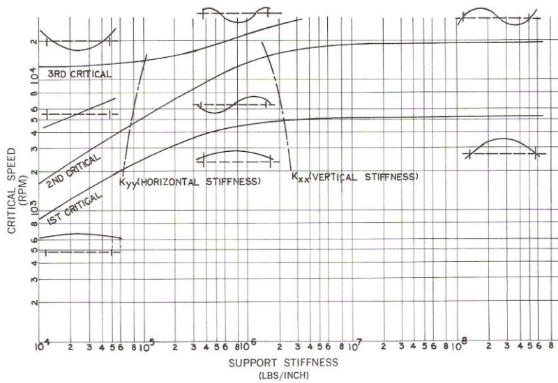
Undamped Critical Speed Map
