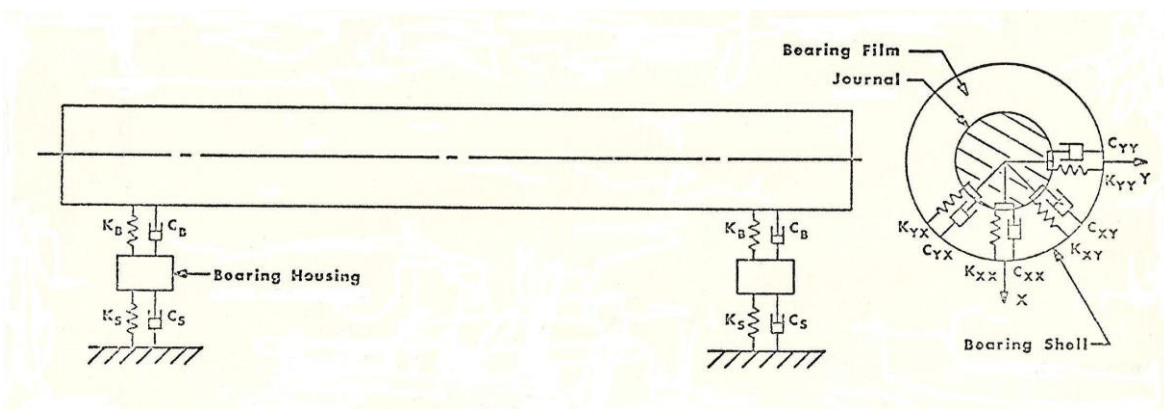
Rotor Bearing System
