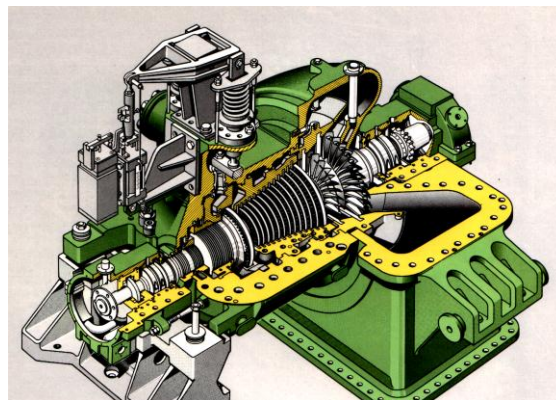
Condensing Steam Turbine
